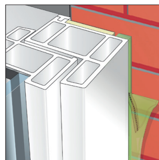
Fig 4: TP601 located between window and reveal.
